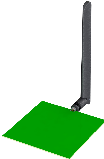
Figure 10. ANT-W63WS4-ccc on Edge of Ground Plane, Bent 90 Degrees (Edge-Bent)
