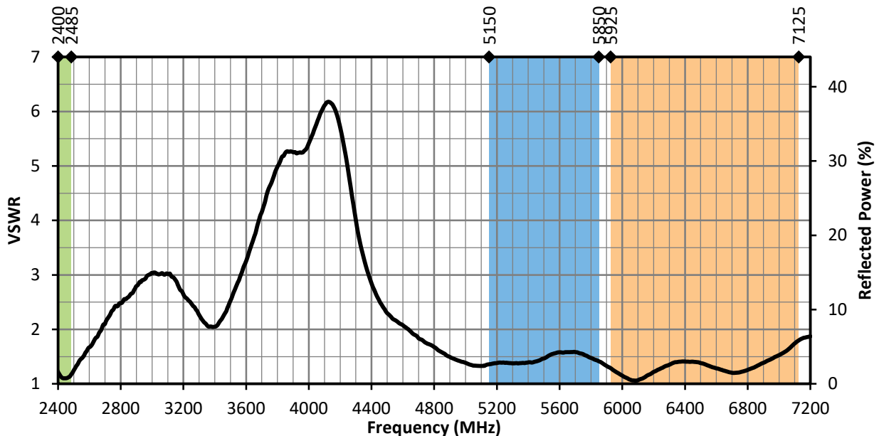
Figure 4. ANT-W63WS4-ccc VSWR, Straight
