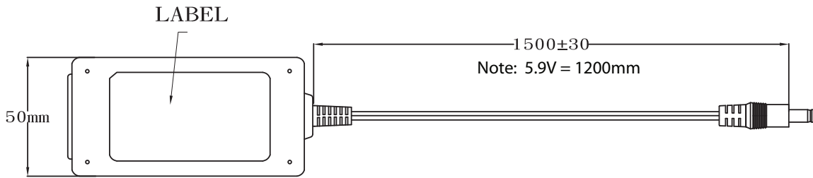
BOTTOM VIEW
