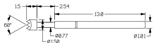
P19-4021 Serrated Head
