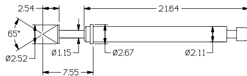
P25-7017 Needle Head 2.54mm Centre
