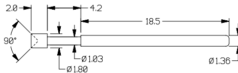
P25-1223 Concave Head
