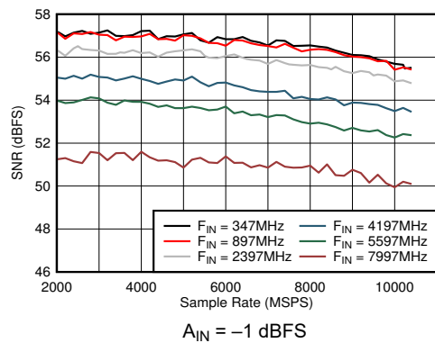
A_{IN} = -1\text{ dBFS} Figure 6-29. DES Mode: SNR vs Sample Rate and Input Frequency
