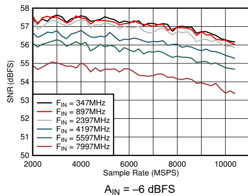
A_{IN} = -6\text{ dBFS} Figure 6-30. DES Mode: SNR vs Sample Rate and Input Frequency
