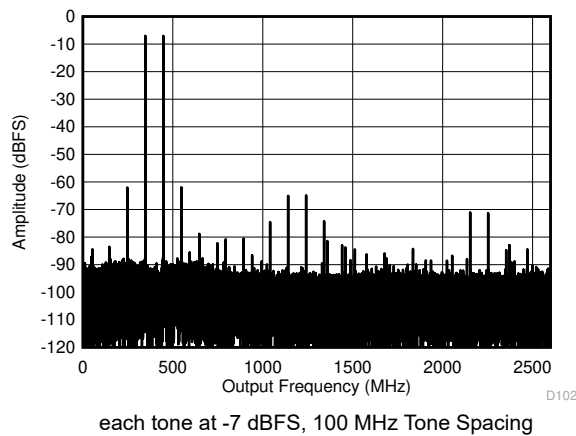
each tone at -7 dBFS, 100 MHz Tone Spacing Figure 6-27. Dual Channel Mode: Two Tone FFT at 5597 MHz
