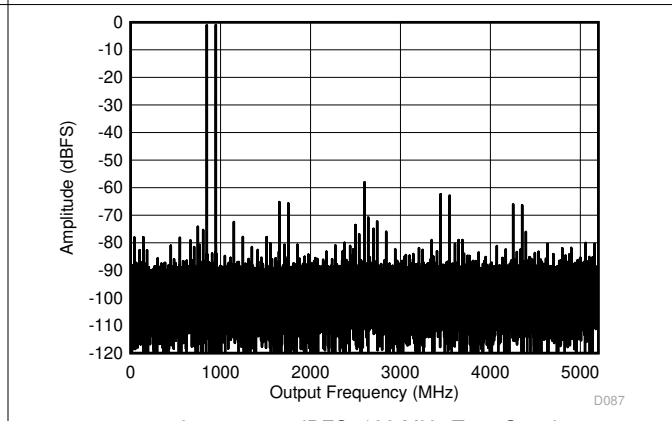
Figure 6-12. DES Mode: Two Tone FFT at 897 MHz
