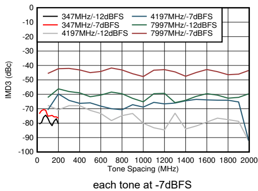
Figure 6-103. DES Mode: IMD3 vs Tone Spacing
