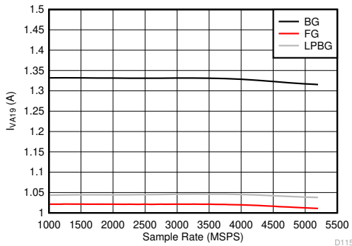
Figure 6-133. Dual Channel Mode: I_{VA19} vs Sample Rate
