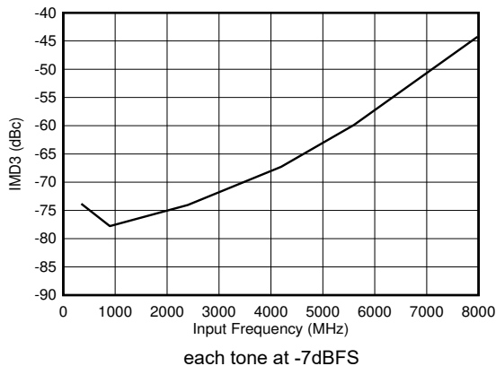
Figure 6-101. DES Mode: IMD3 vs Input Frequency
