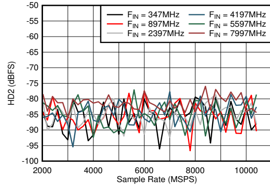
Figure 6-38. DES Mode: HD2 vs Sample Rate and Input Frequency
