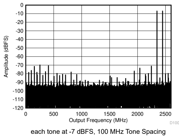
each tone at -7 dBFS, 100 MHz Tone Spacing Figure 6-25. Dual Channel Mode: Two Tone FFT at 2397 MHz
