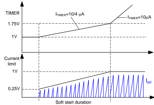
Figure 6: Soft Start
