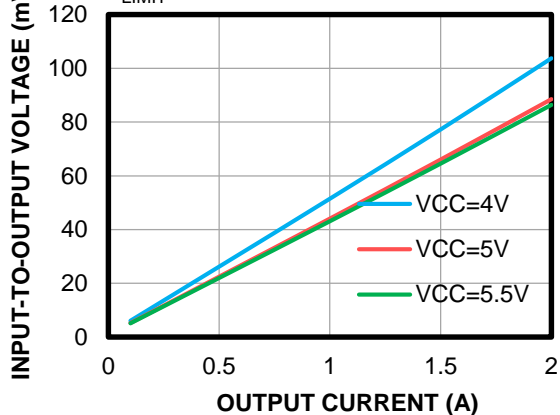
Input-to-Output Voltage vs. Output Current
