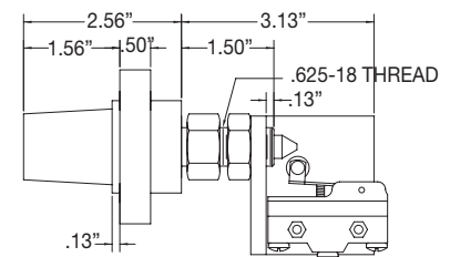
Female Receptacle Assembly With Interlock Switch
