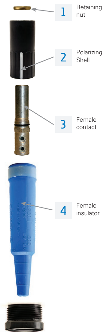
Female Plug Assembled length is 8 3/4"
