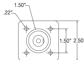
Female Receptacle Assembly With Interlock Switch
