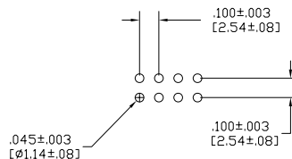
RECOMMENDED HOLE PATTERN
