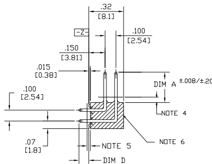
SECTION Z-Z
